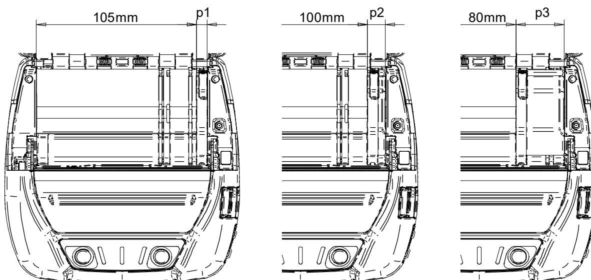
Figure 13-2 Partition Plate and Attachment Position
