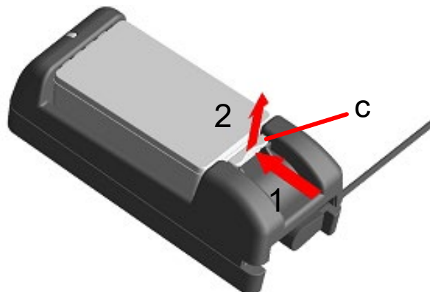
Figure 17-7 Battery Pack Removal from Battery Charger
