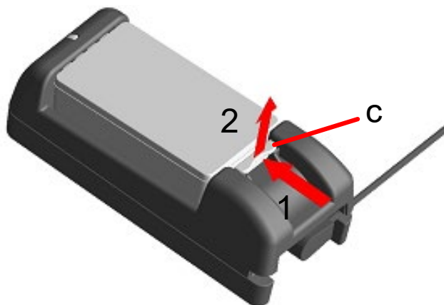
Figure 18-7 Battery Pack Removal from Battery Charger
