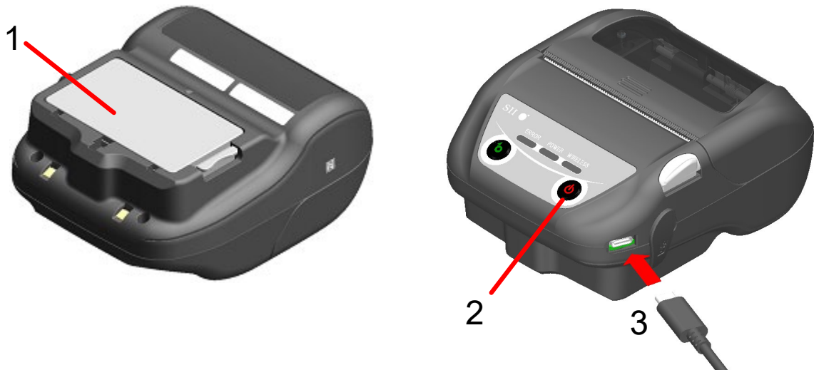
Figure 16-1 Charging in Power On Charging Mode from USB AC Adapter
