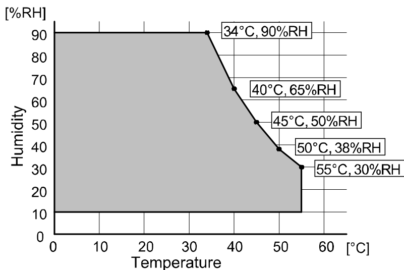
Figure 21-1 Operating Temperature and Humidity Range (Printing)
