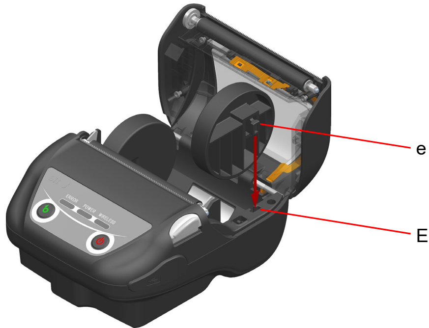
Figure 14-2 Installing Partition Plate (2)
