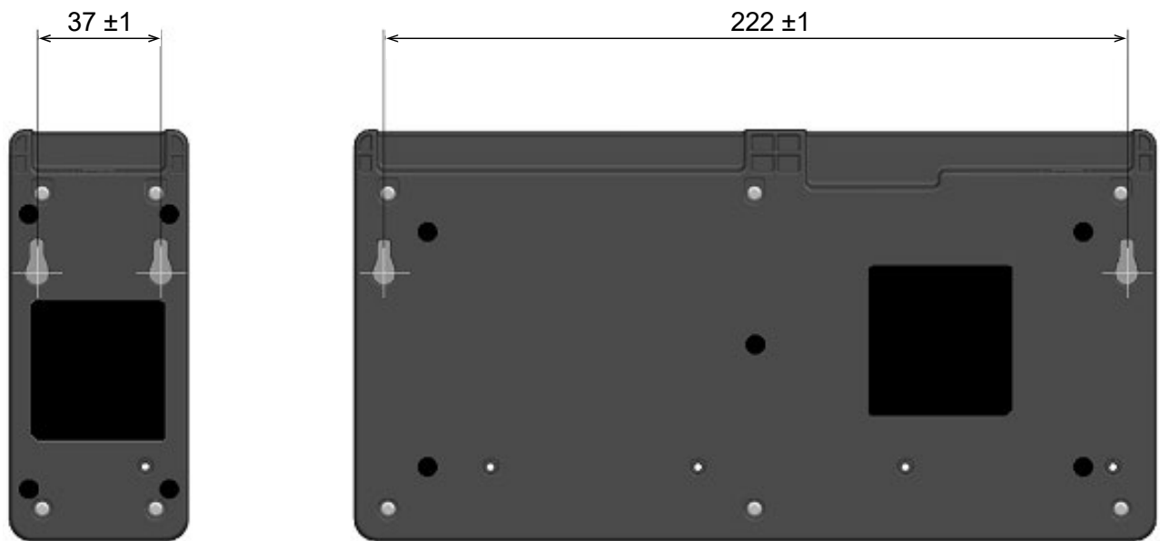
Figure 18-8 Bottom of Battery Charger
