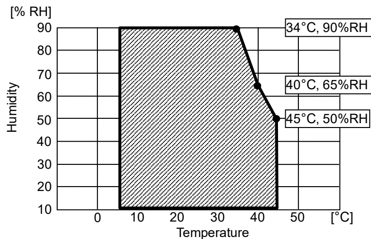
Figure 16-1 Operating Temperature and Humidity Range
