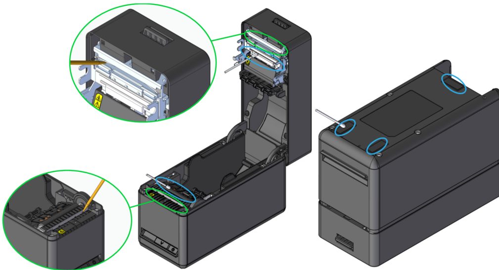
Figure 13-1 Cleaning Thermal Head / Platen / Rubber Feet / Cutter
